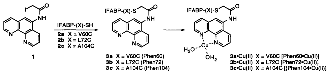
Figure 1. Procedure employed for the preparation and metallation of IFABP-phenanthroline conjugates.
