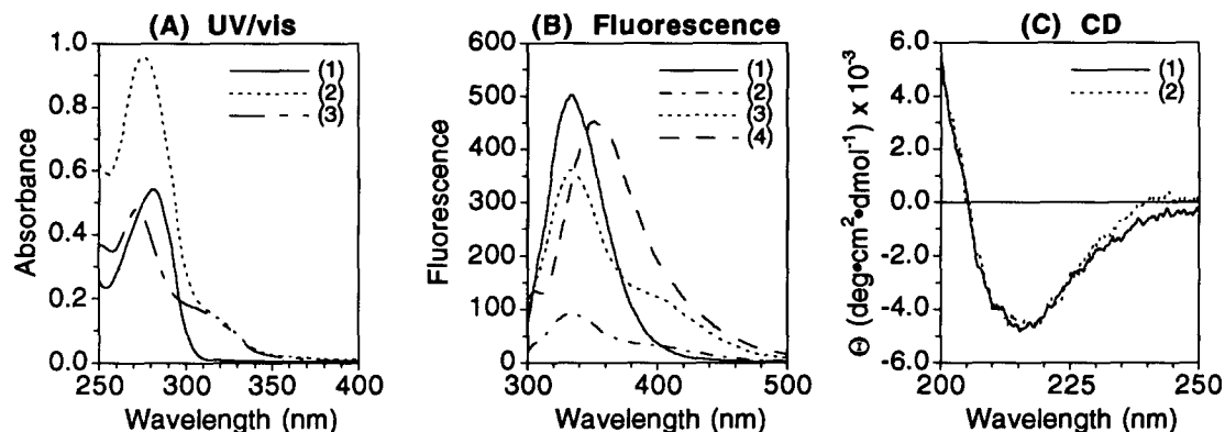
Figure 2. Spectroscopic properties of the L72C (2b) and Phen72 (3b) proteins. (A) UV/vis spectra obtained using 25 \mu M protein in Tris buffer (50 mM, pH 7.4). (1) Spectrum of L72C protein. (2) Phen72. (3) Difference spectrum of (2) minus (1). (B) Fluorescence spectra obtained using 1.0 \mu M protein in Tris buffer (50 mM, pH 7.4) at 25 ^{\circ} C with \lambda_{\text{exc}} = 275 nm and slit widths of 5.0 nm (excitation) and 4.0 nm (emission). (1) Emission spectrum of L72C protein. (2) Phen72. (3) Same as (2) but with slit widths of 7.5 nm (excitation and emission). (4) Same as (3) but obtained in 2.5 M guanidine \cdot HCl. (C) Circular dichroism spectra obtained using 15 \mu M protein in Tris buffer (50 mM, pH 7.4). (1) Spectrum of L72C protein. (2) Phen72.
